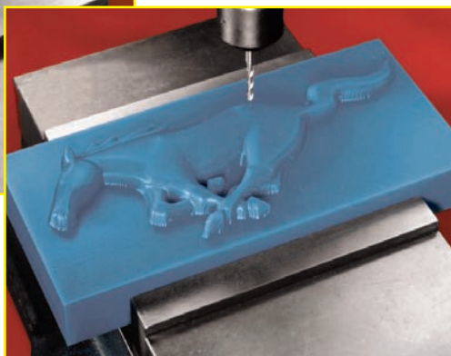
◀ Exact Duplicate Cut without Programming
