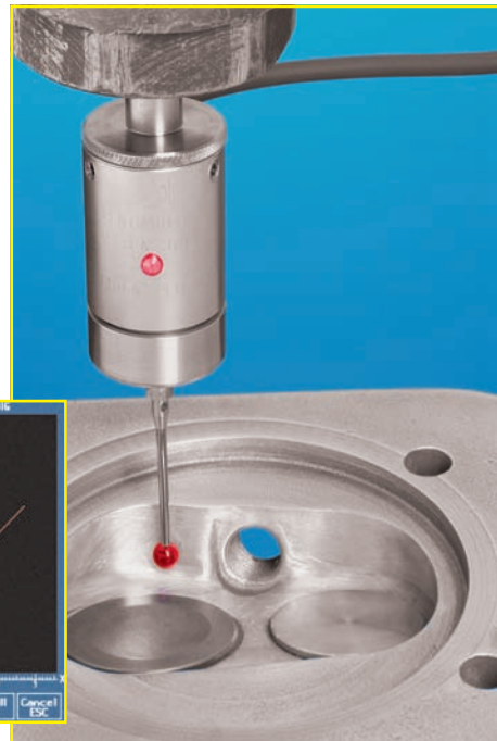
Digitizing a Cylinder Head
