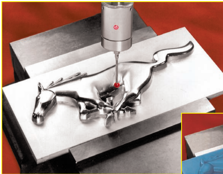
▲ Complex Surface Being Digitized with Centroid's DP-4 All-Surface Probe
